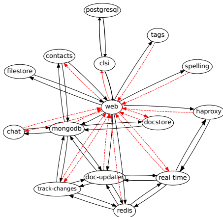
Figure 6. Relations between components based on Granger Causality in ShareLatex. The dashed lines denote relationships with metric http-requests_Project_id_GET_mean .
